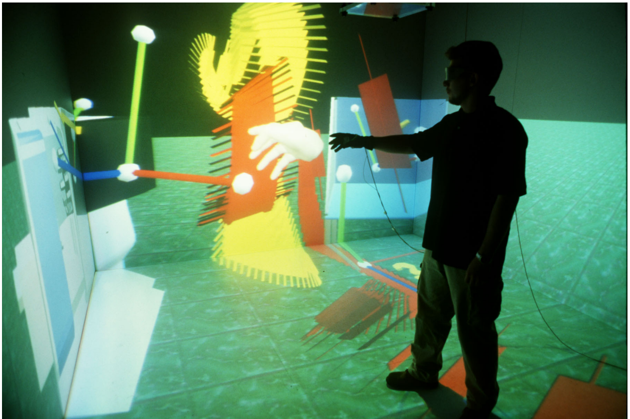
Figure 10. VRSpatial: Congruences
