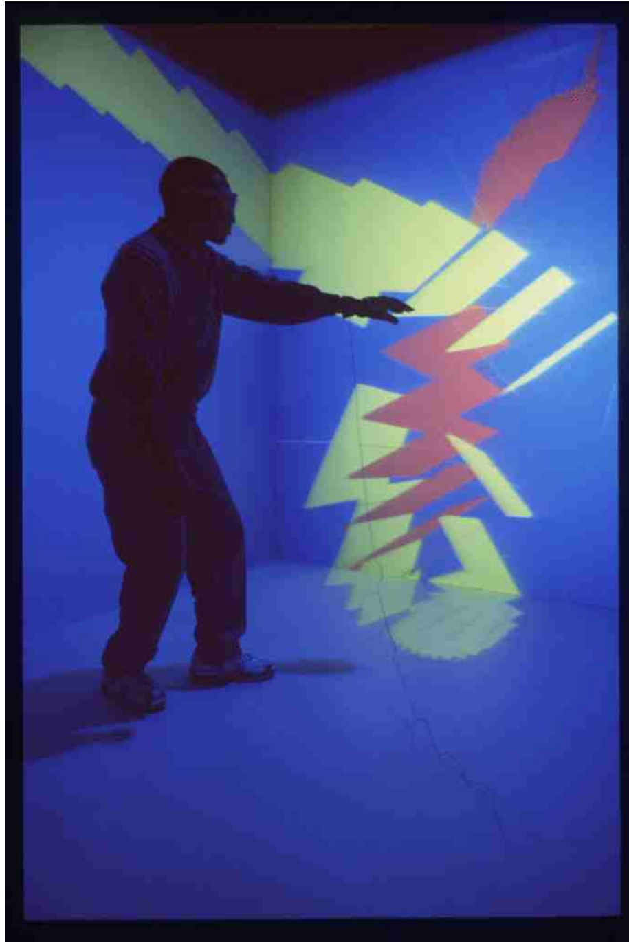
Figure 6. 2001 Congruence Visualization
