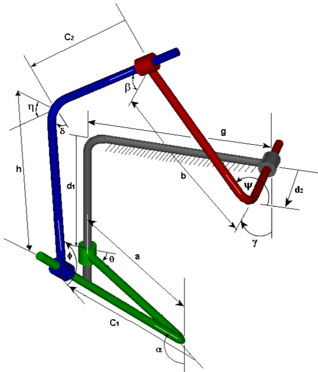
Figure 1. A Spatial 4C Mechanism
